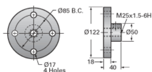
Top Plate (optional): 9000-EM-02
