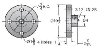
Top Plate (optional): 9000-00-13
