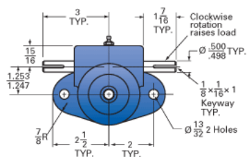
Top Plate (optional): 9000-00-11
