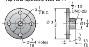
Top Plate (optional): 9000-00-11
