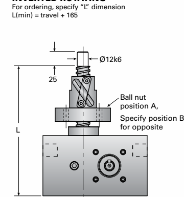
EM1C-BSJ-UR UPRIGHT & INVERTED ROTATING
