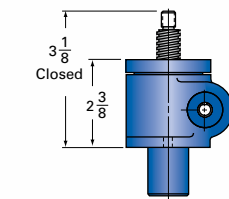
MJ-xx-UK UPRIGHT KEYED
