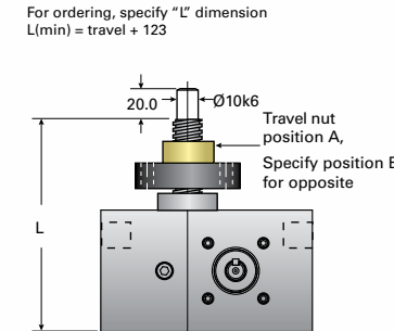
EM05C-MSJ-UR UPRIGHT & INVERTED ROTATING
