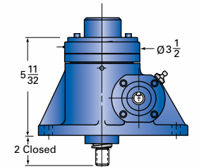
2R-MSJ-IK INVERTED KEYED
