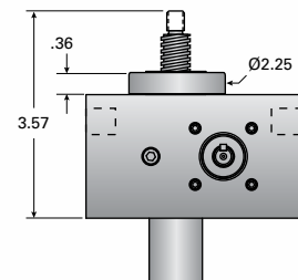
MJABC-xx-U UPRIGHT ANTI-BACKLASH
