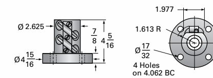
10HL-BSJ Ball Nut and Flange
