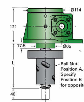
EM5-BSJ-IR INVERTED ROTATING For ordering, specify "L" dimension L(min) = travel + 157
