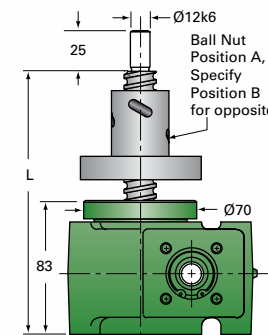
EM1-BSJ-UR UPRIGHT ROTATING For ordering, specify "L" dimension L(min) = travel + 164
