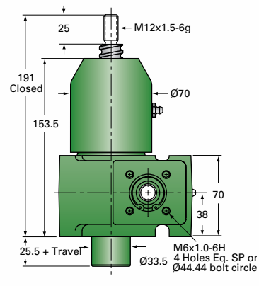
EM1-BSJ-U UPRIGHT
