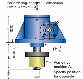
2R-MSJ-IR INVERTED ROTATING
