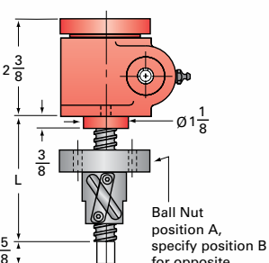
0.5-BSJ-IR & 0.5HL-BSJ-IR INVERTED ROTATING FOR ORDERING: Specify "L" dimension L (min) = Travel + 2 5/8
