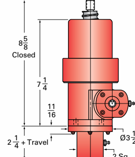
3-BSJ-UK UPRIGHT KEYED
