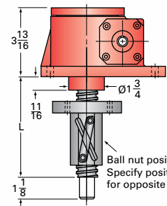
2.5HL-BSJ-IR INVERTED ROTATING
