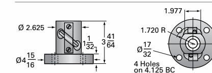
10HL-BSJ Ball Nut and Flange
