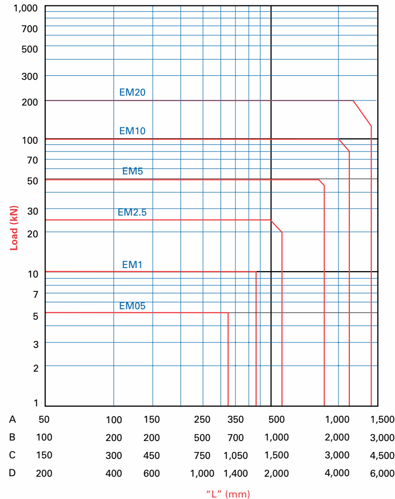
"L" (mm) Metric Ball Screw Jack
