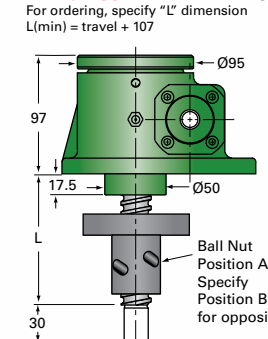
EM2.5-BSJ-IR INVERTED ROTATING
