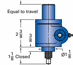
MJ-xx-I INVERTED
