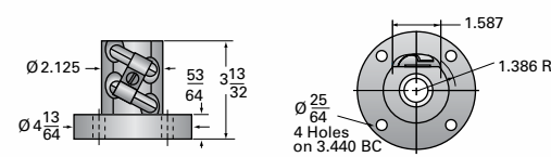
3-BSJ Ball Nut and Flange
