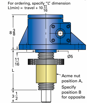
35-MSJ-IR INVERTED ROTATING
