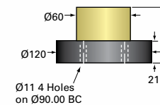
EM5-MSJ Travel Nut and Flange
