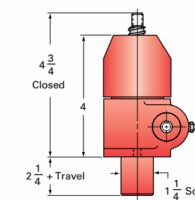
0.5-BSJ-IK & 0.5HL-BSJ-IK UPRIGHT KEYED
