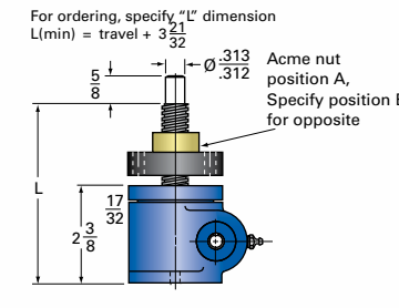
MJ-xx-UR UPRIGHT ROTATING
