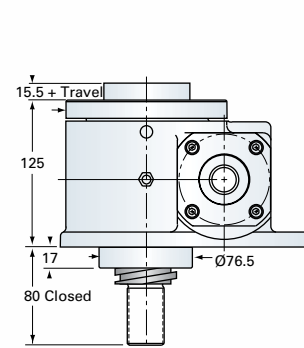
EM10-MSJ-I INVERTED
