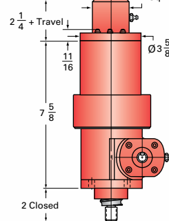
3-BSJ-IK INVERTED KEYED
