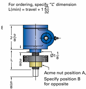
MJ-xx-IR INVERTED ROTATING
