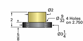
2-MSJ Acme Nut and Flange
