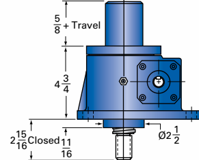
5-MSJ-I INVERTED
