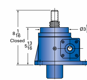
5-MSJ-UK UPRIGHT KEYED
