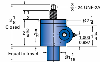
MJ-xx-U UPRIGHT
