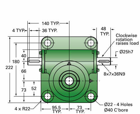
EM10-BSJ TOP VIEW
