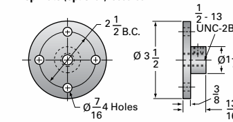
Motor Mounts
