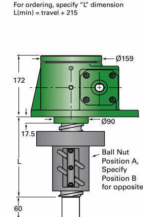
EM20-BSJ-IR INVERTED ROTATING
