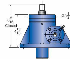
2R-MSJ-UK UPRIGHT KEYED
