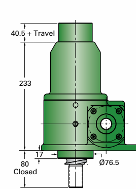
EM10-BSJ-I INVERTED
