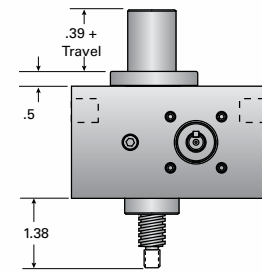
1ABC-MSJ-I INVERTED ANTI-BACKLASH
