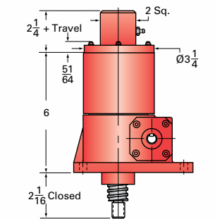
2.5HL-BSJ-IK INVERTED KEYED
