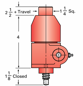
0.5-BSJ-IK & 0.5HL-BSJ-IK INVERTED KEYED
