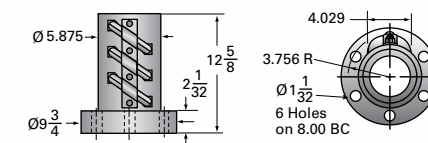
75-BSJ Ball Nut and Flange
