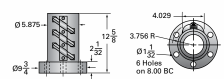
100-BSJ Ball Nut and Flange
