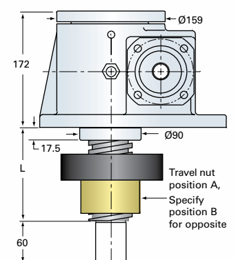
EM20-MSJ-IR INVERTED ROTATING
