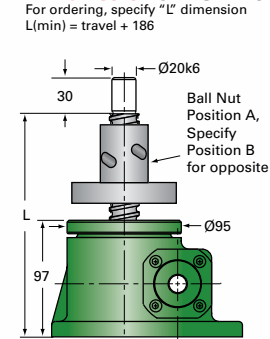
EM2.5-BSJ-UR UPRIGHT ROTATING
