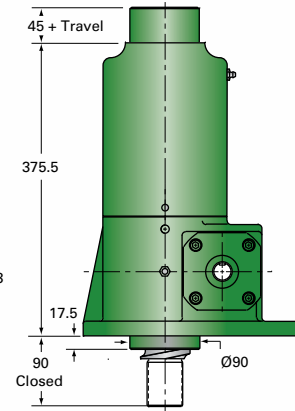
EM20-BSJ-I INVERTED
