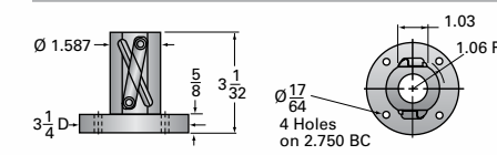
2.5HL-BSJ Ball Nut and Flange
