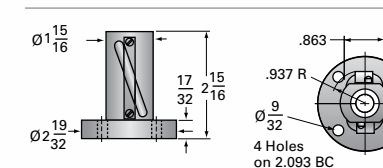
1CHL-BSJ Ball Nut and Flange
