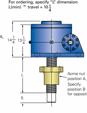
100-MSJ-IR INVERTED ROTATING
