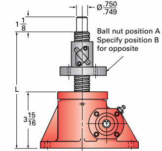
2R-BSJ-UR UPRIGHT ROTATING
