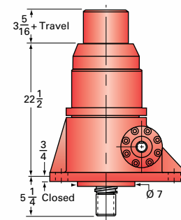
75-BSJ-I INVERTED
