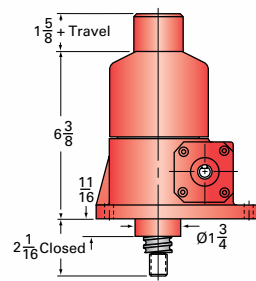
2.5HL-BSJ-I INVERTED
