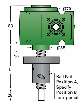
EM1-BSJ-IR INVERTED ROTATING For ordering, specify "L" dimension L(min) = travel + 90
