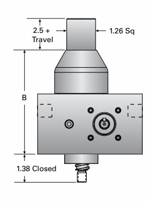
1C-BSJ-IK & 1CHL-BSJ-IK INVERTED KEYED
