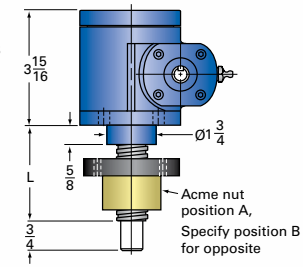
2-MSJ-IR INVERTED ROTATING
