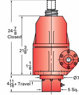
50-BSJ-UK UPRIGHT KEYED
