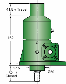
EM2.5-BSJ-I INVERTED
