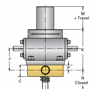
MSJ-I (Machine Screw Inverted)
